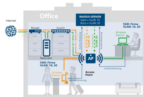
Fig. 5: Dynamic VLAN
