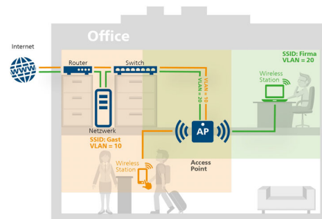
Fig. 4: Static VLAN
