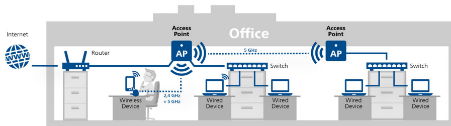
Fig. 3: WDS bridge
