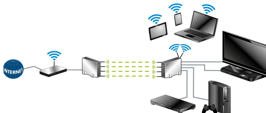
Fig. 6: Setting up the devolo GigaGate connections
