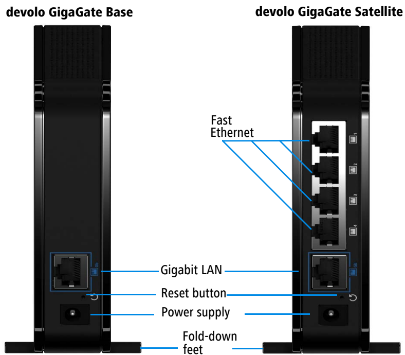
Fig. 4: Rear side of the GigaGate device
